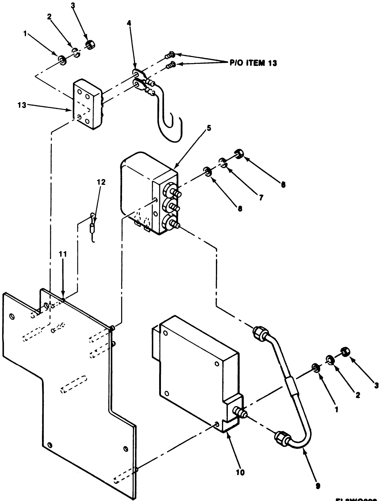
Figure 15. BITE Assembly, RF
