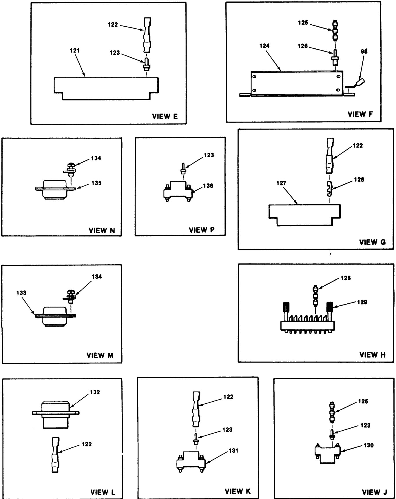
Figure 2. Receiver-Transmitter RT-1149(V)1/ALQ-136(V) (sheet 5 of 5).
