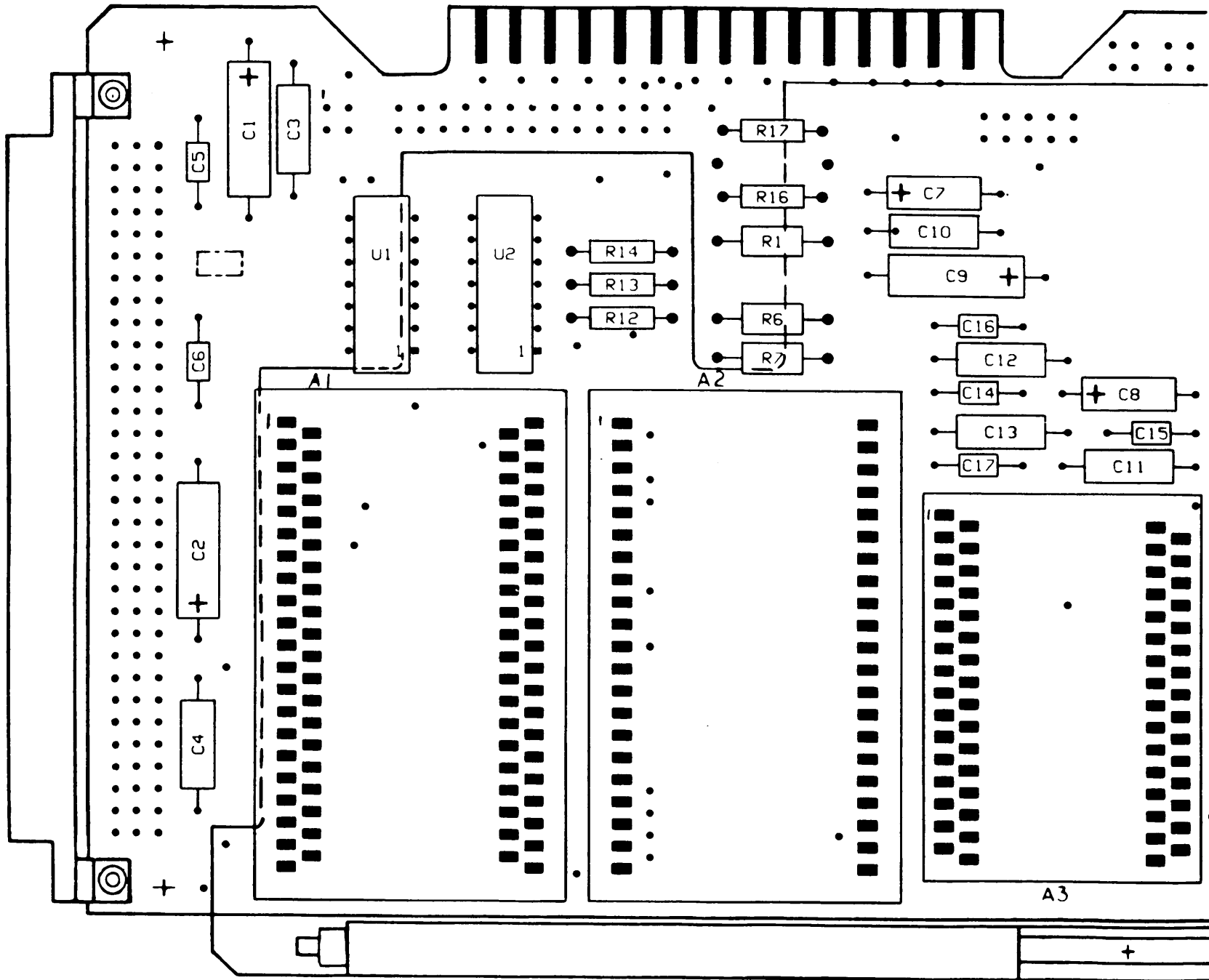
Figure 6. Circuit Card Assembly, Supervisory Control (1A4) (Sheet 1 of 3)
