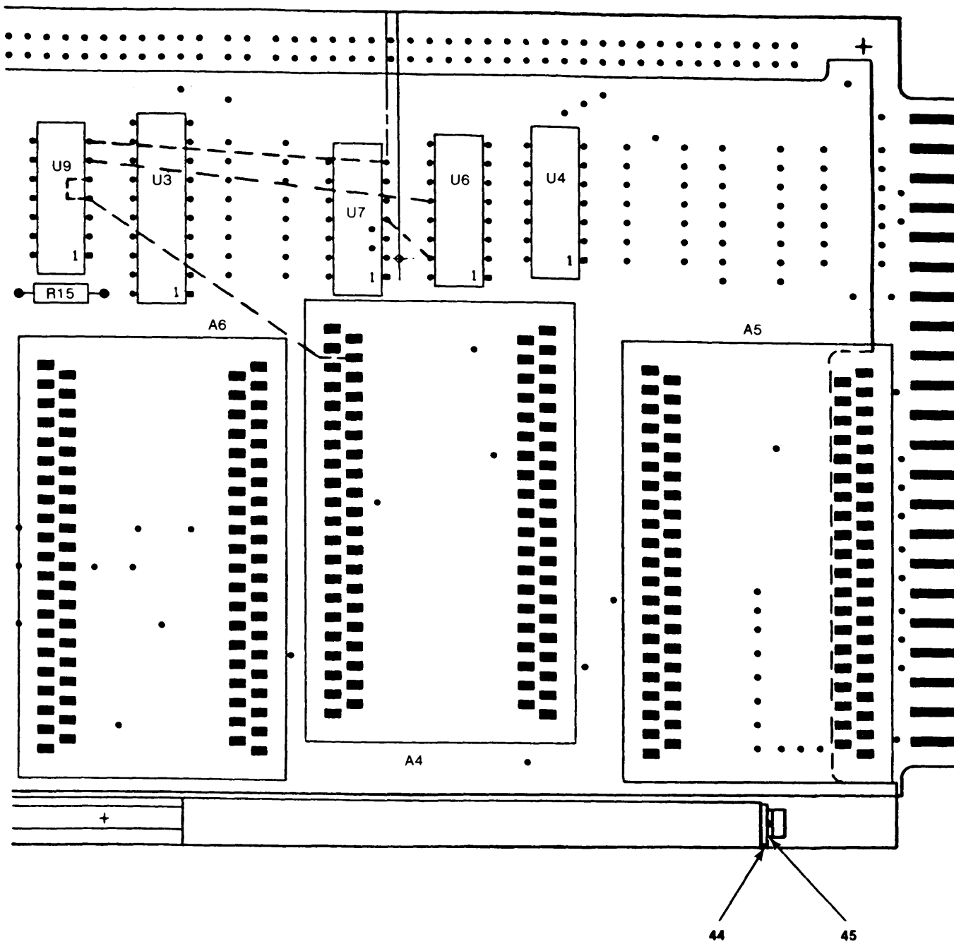
Figure 6. Circuit Card Assembly, Supervisory Control (1A4) (Sheet 2 of 3)
