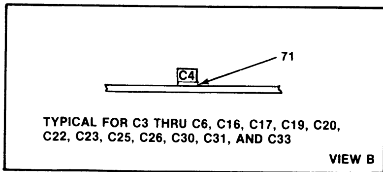
Figure 5. Circuit Card Assembly, Mod Recovery (1A3) (Sheet 1 of 2)
