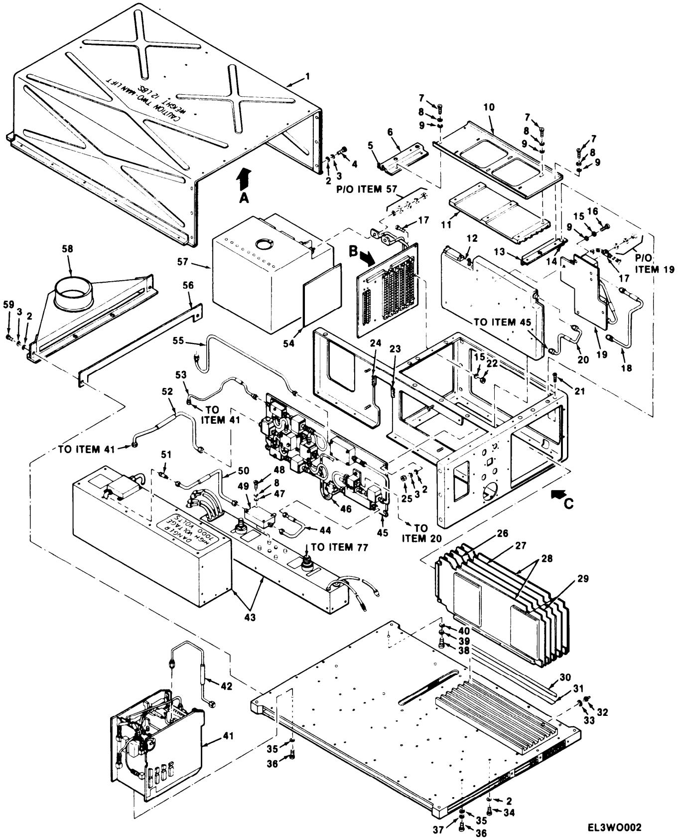
Figure 2. Receiver-Transmitter RT-1149(V)1/ALQ-136(V) (Sheet 1 of 5).
