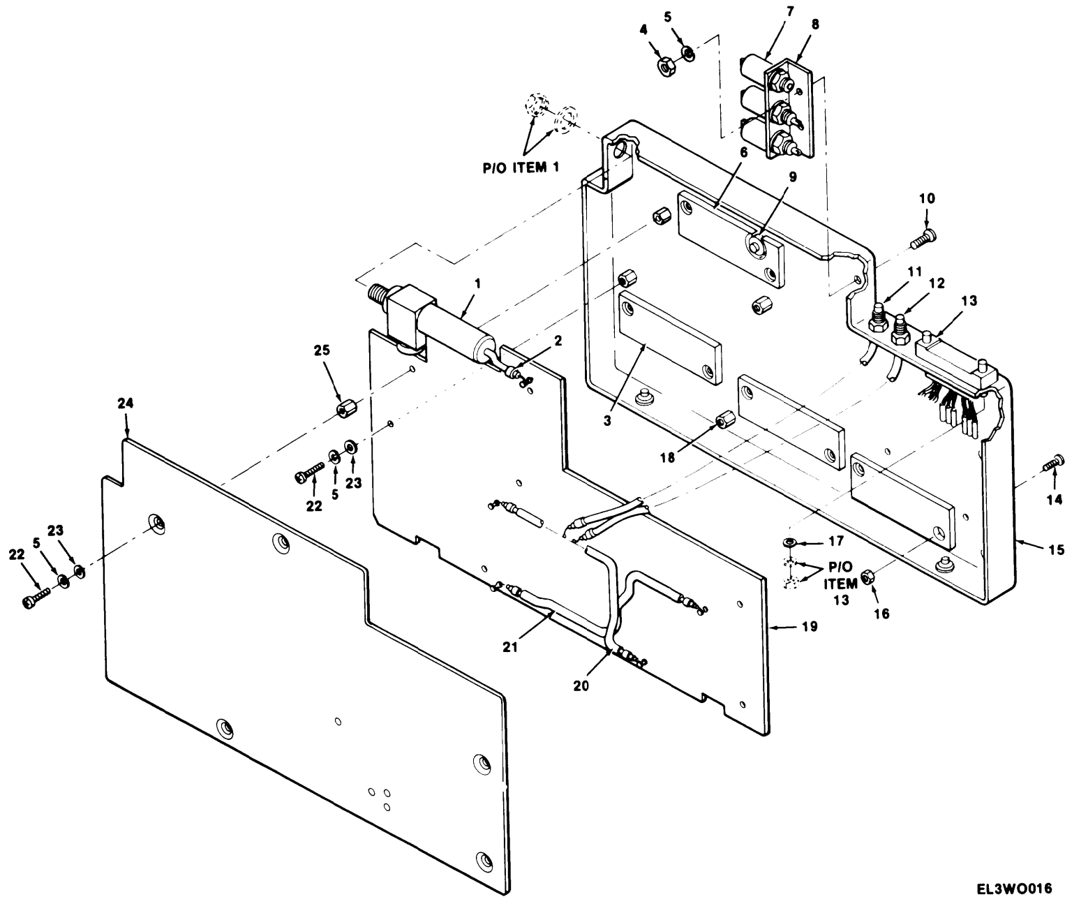
Figure 7. Receiver Assembly
