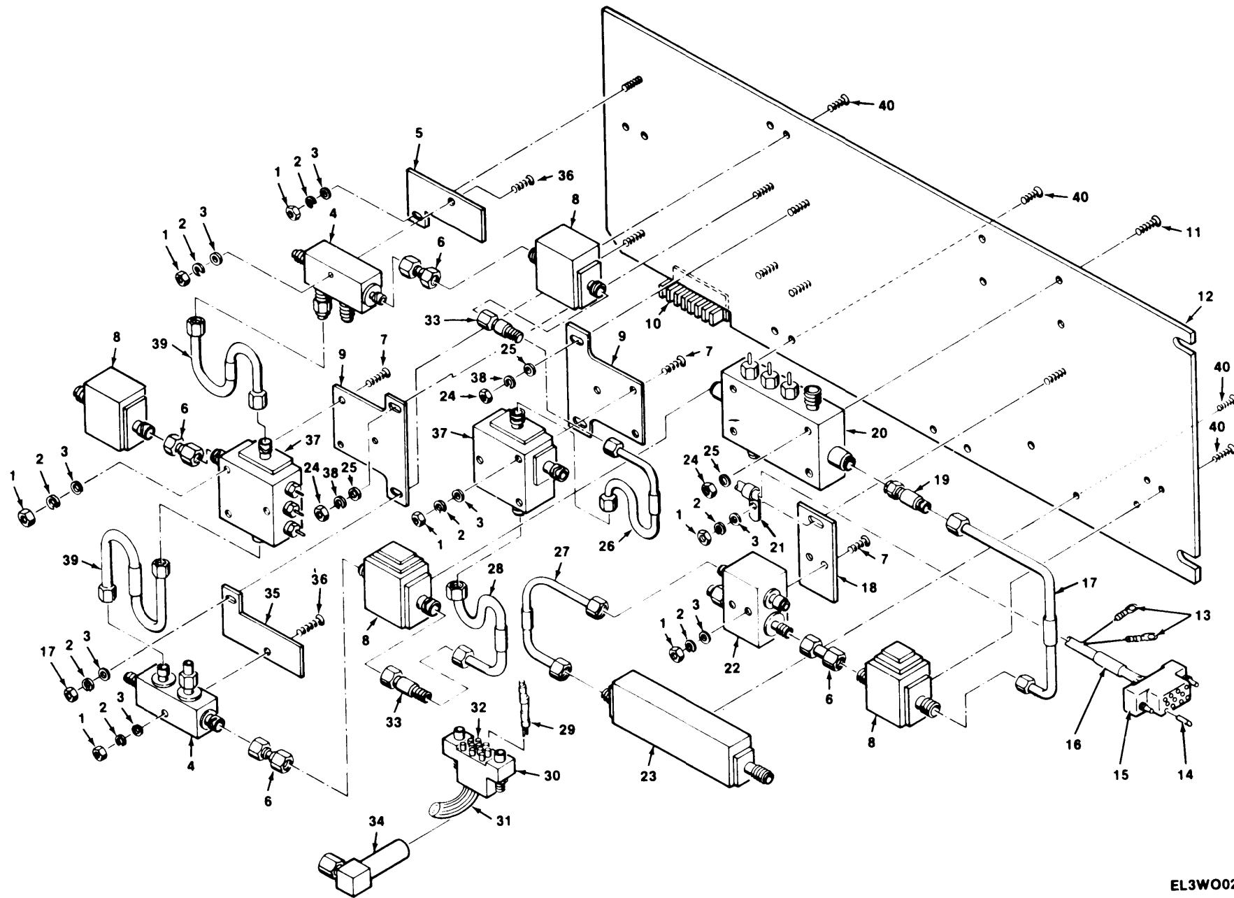
Figure 14. RF Tray Assembly
