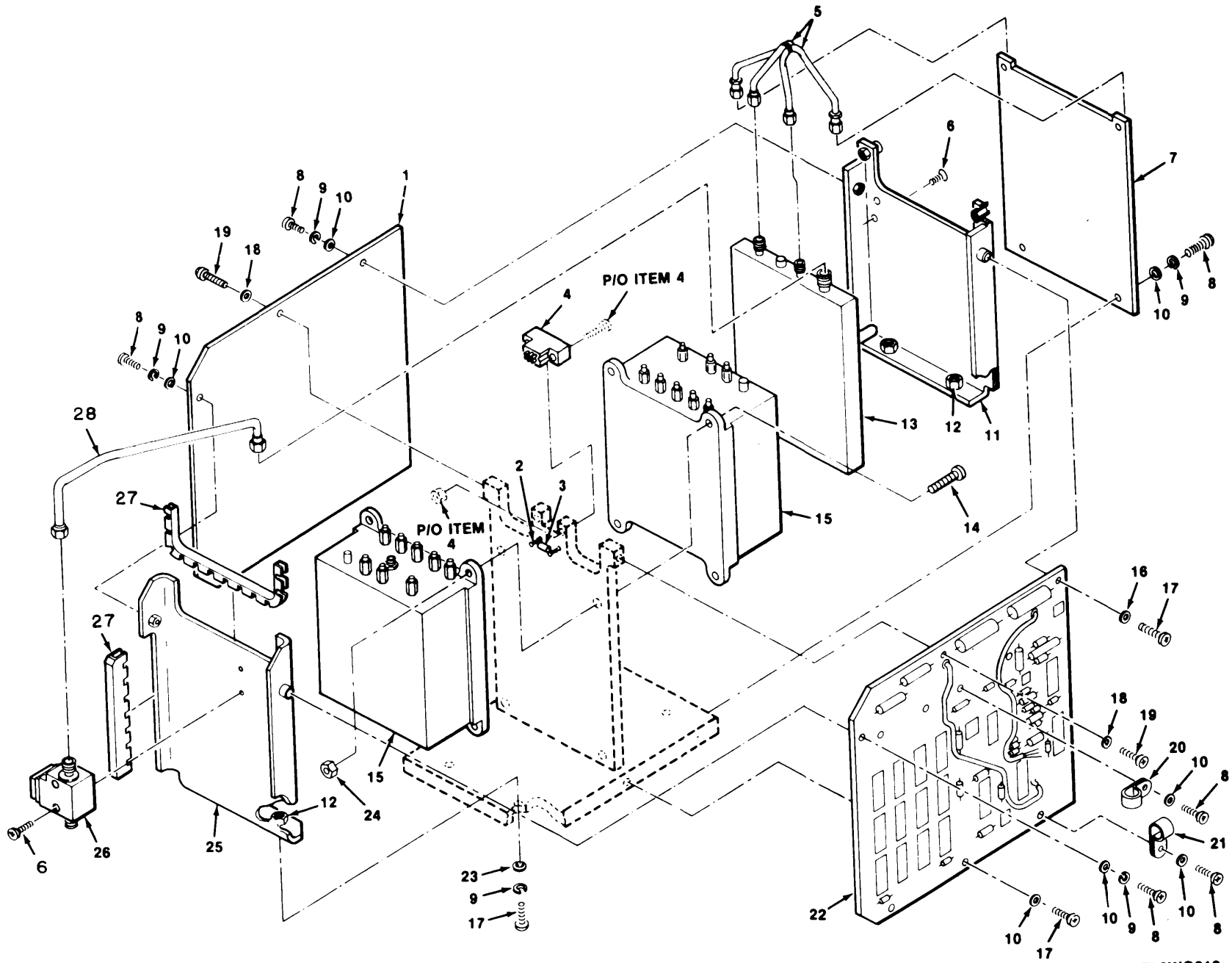
Figure 9. Oscillator Assembly
