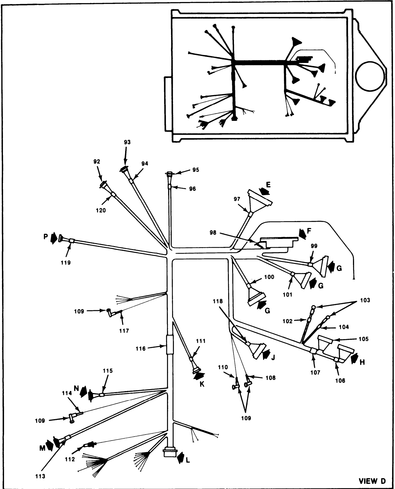
Figure 2. Receiver-Transmitter RT-1149(V)1/ALQ-136(V) (Sheet 4 of 5).
