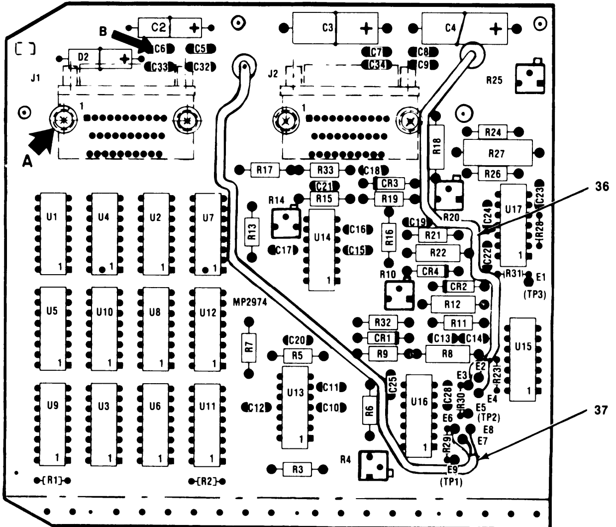
Figure 12. Circuit Card Assembly, VCO-AGC-D/A (Sheet 1 of 2)
