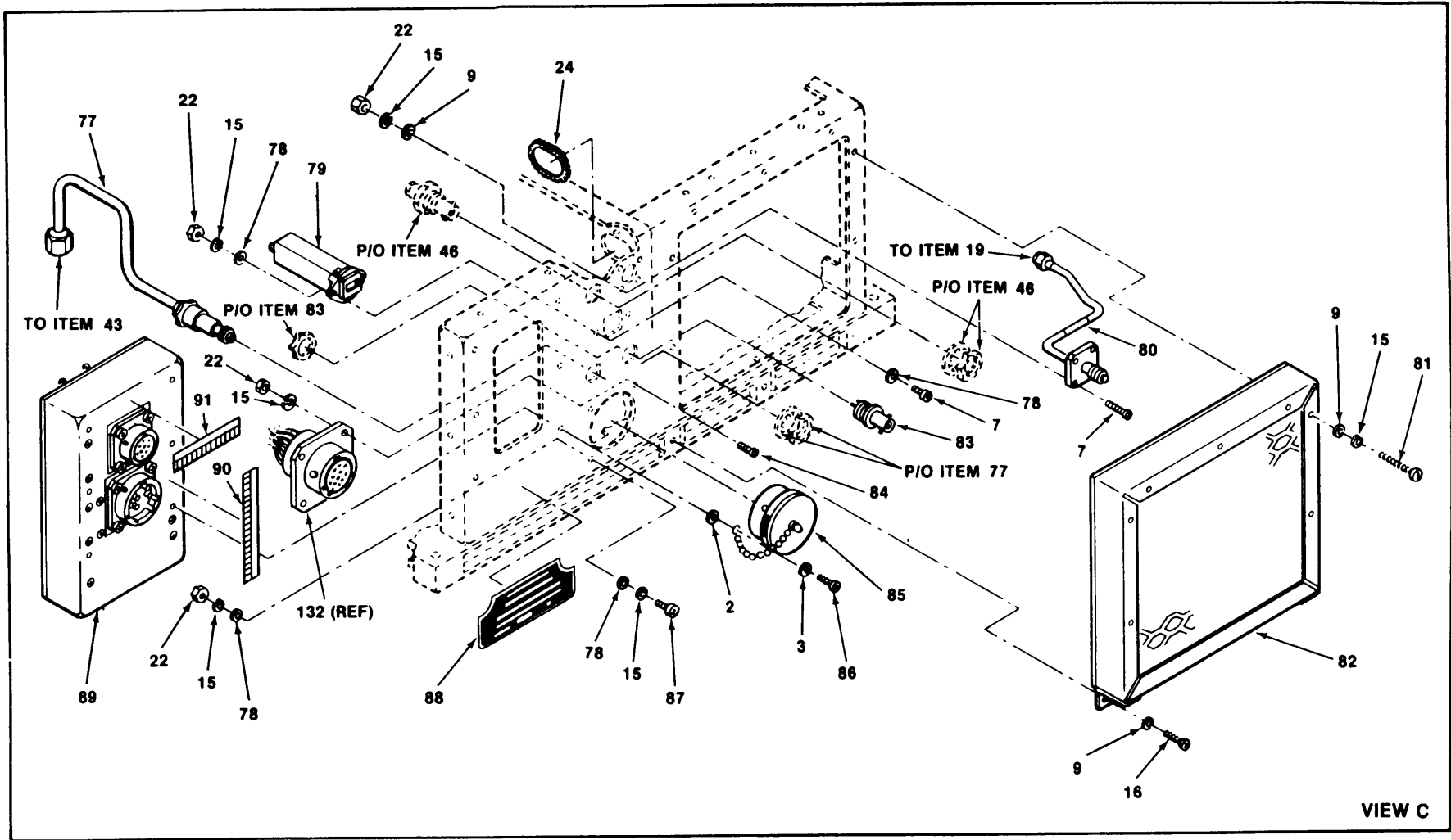
Figure 2. Receiver-Transmitter RT-1149(V)1/ALQ-136(V) (Sheet 3 of 5).
